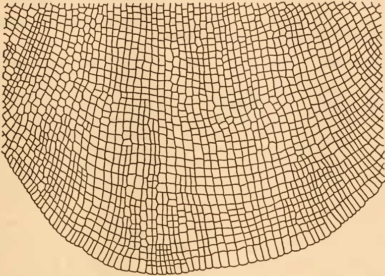
Fig. 1. Spatoglossum Howelii Setchell and Gardner, new species. Apical portion of a frond showing the character of the cells. \times 45 .
